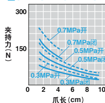
■CKA·CKB·CKD-25AS
