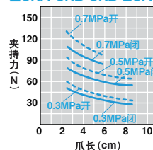
■CKA·CKB·CKD-20AS
