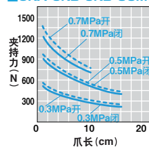
■CKA·CKB·CKD-50MS
